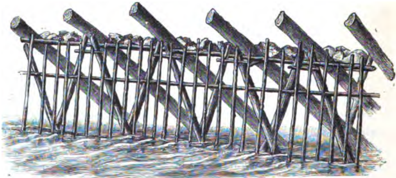
Fig. 262.—Trestle boom.
